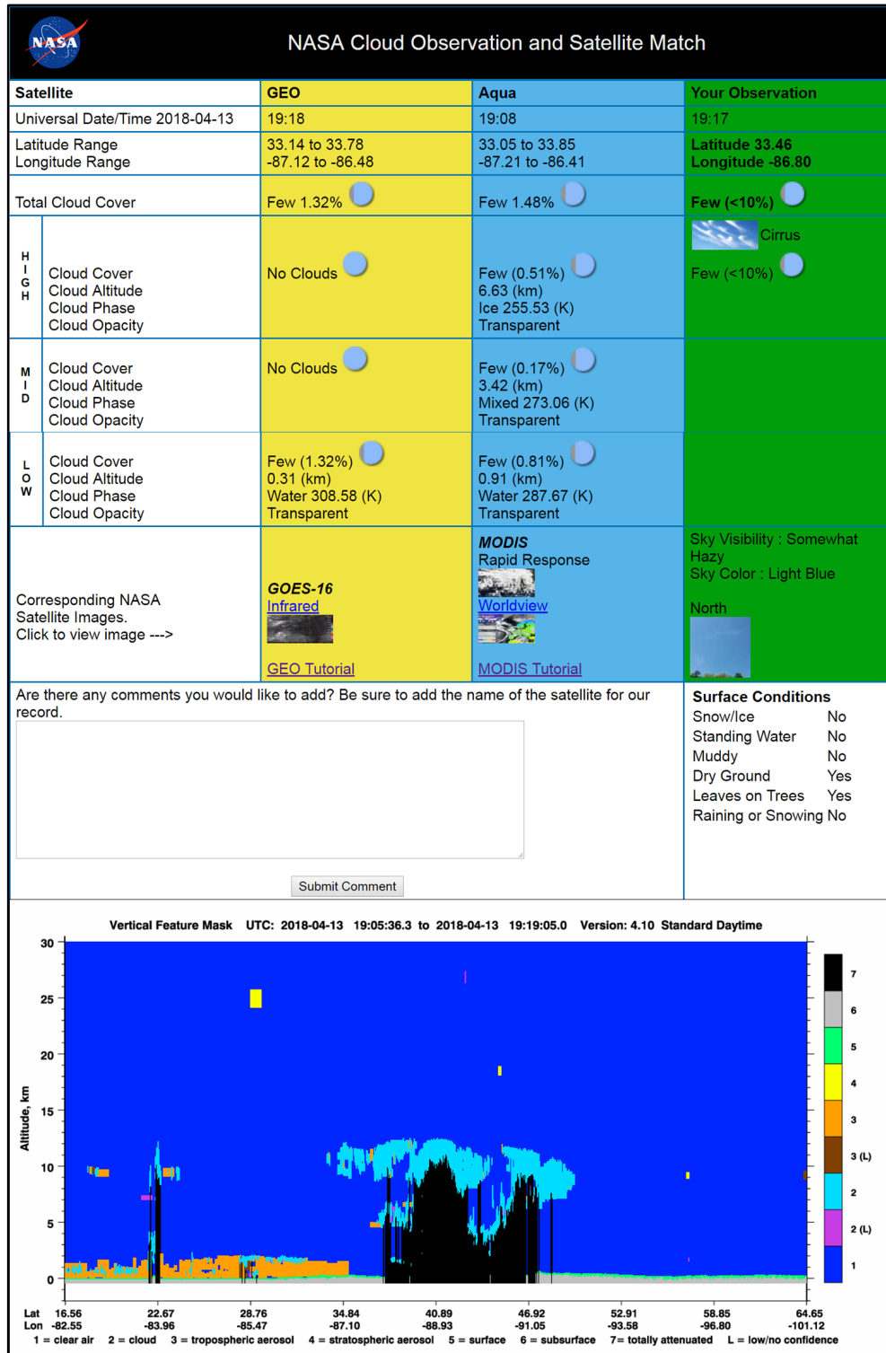
Image 4. Example Ground Observation with Satellite Collocation with CALIPSO
